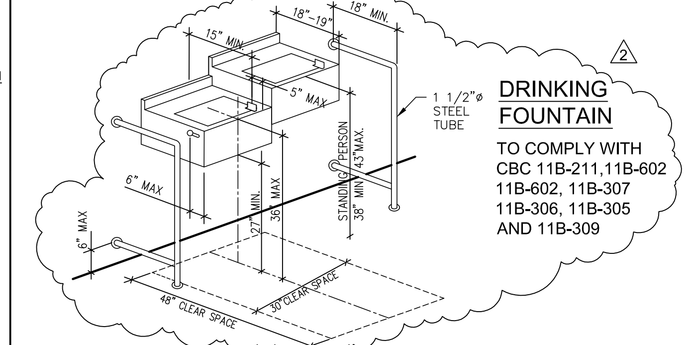
DRINKING FOUNTAINNS SCALE NTS 3
