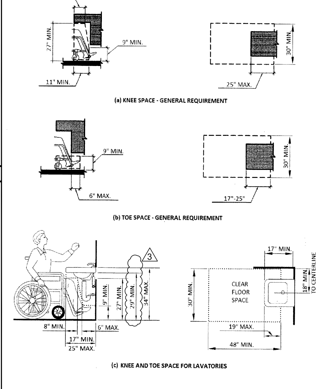
KNEE & TOE SPACE SCALE NTS 4
