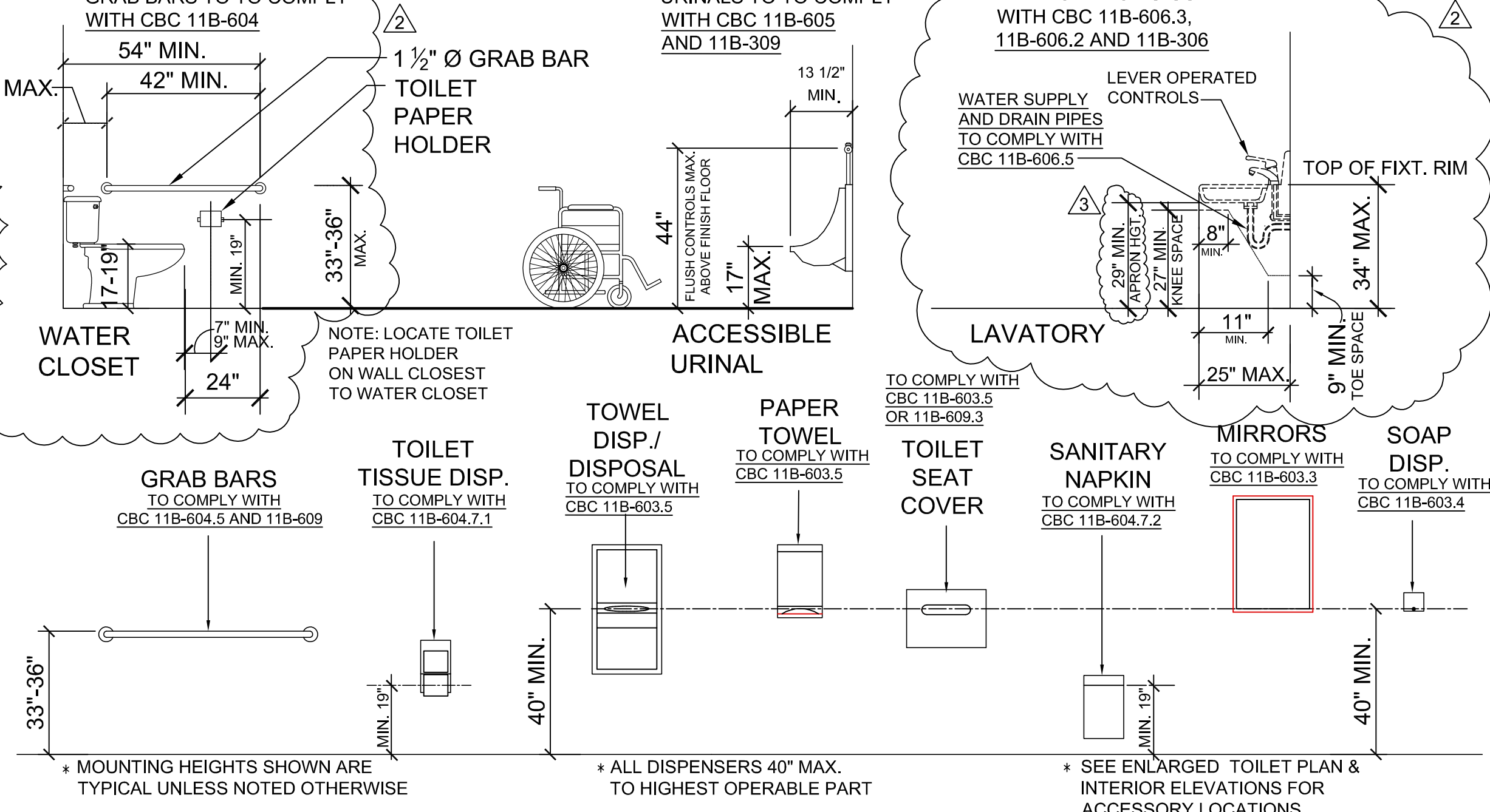
FIXTURE MOUNTING HEIGHTS SCALE NTS 2
