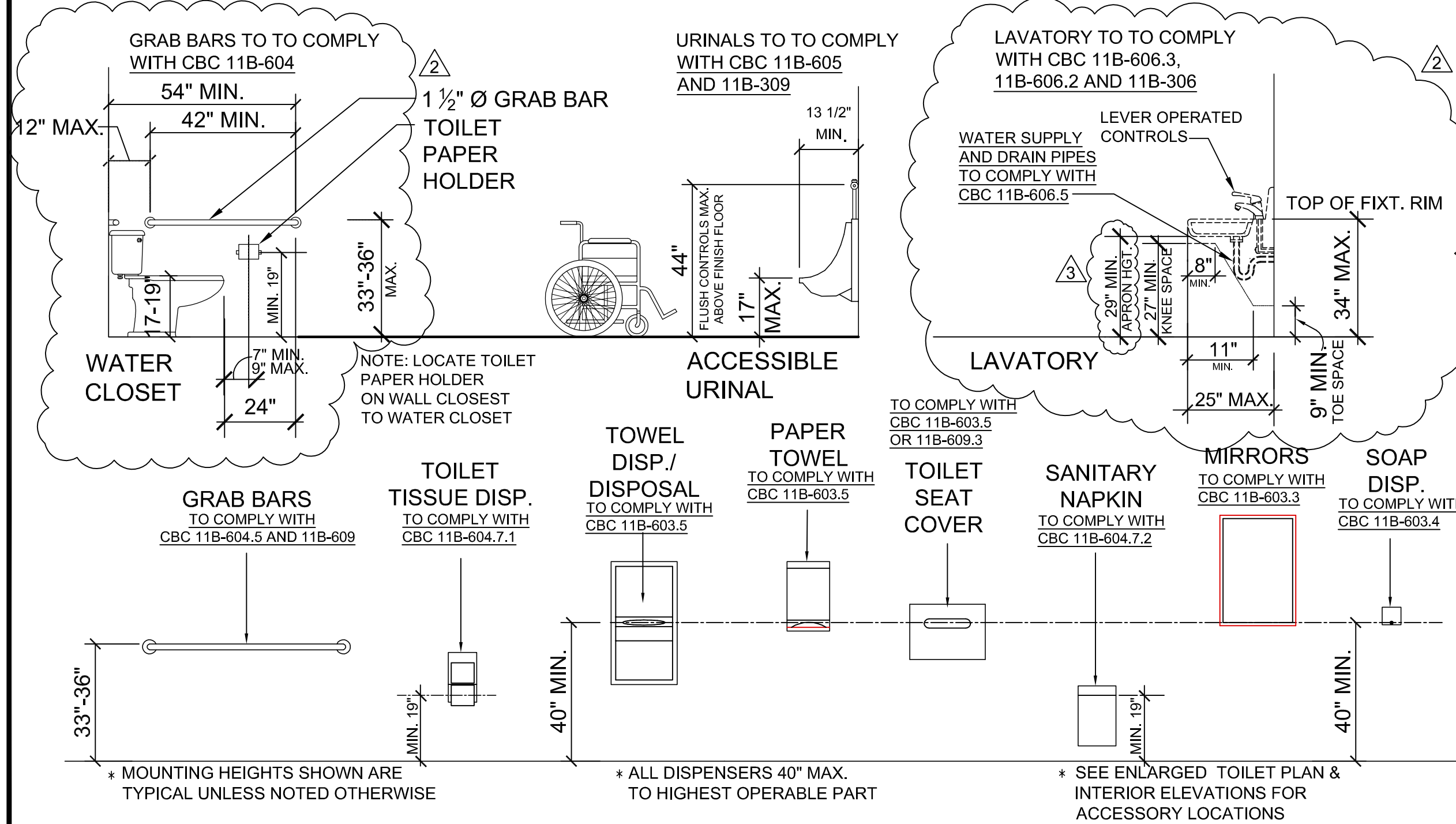
FIXTURE MOUNTING HEIGHTS SCALE NTS 2 DRINKING FOUNTAINS SCALE NTS 3
